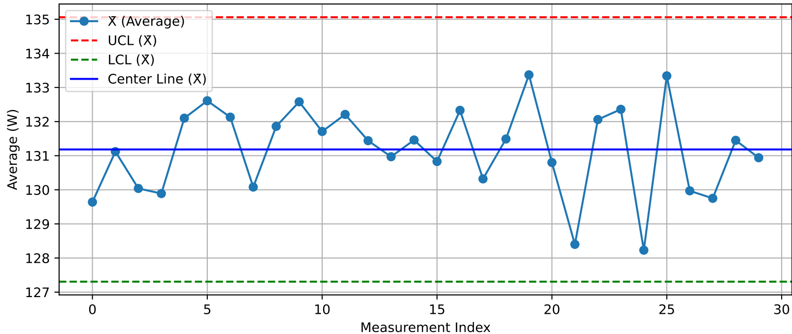
DUT - \bar{X} Chart (T19_Test2@Test.xlsx)
