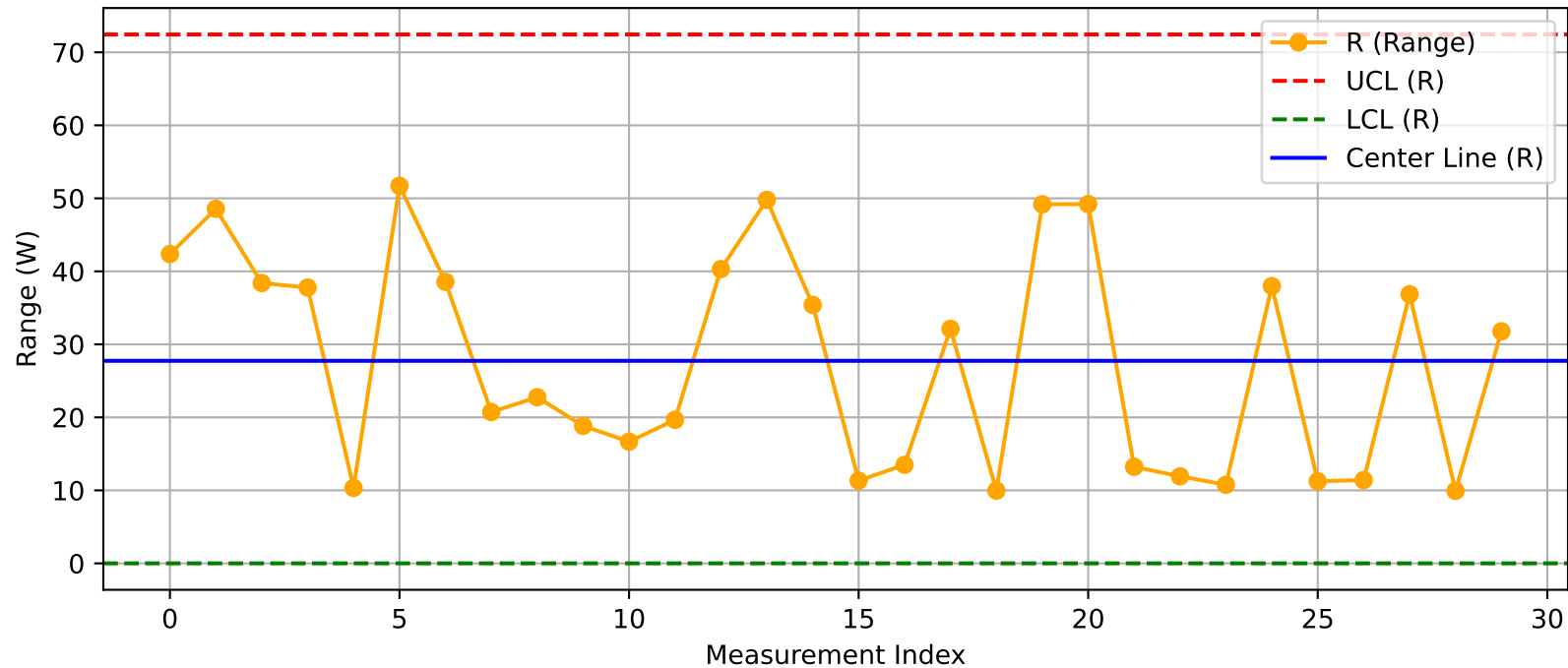
DUT - R Chart (T19_Test2_Xint@Test.xlsx)
