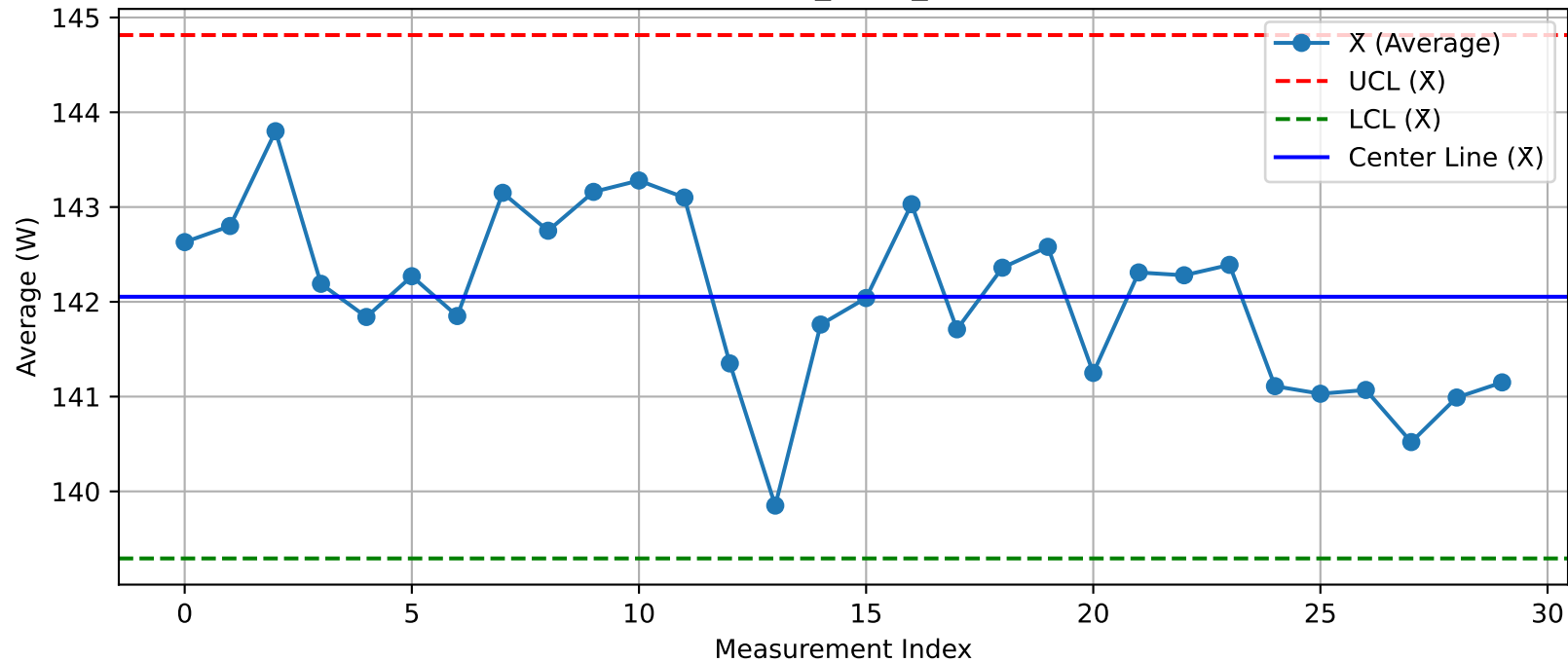
DUT - \bar{X} Chart (T19_Test2_Xint@Test.xlsx)
