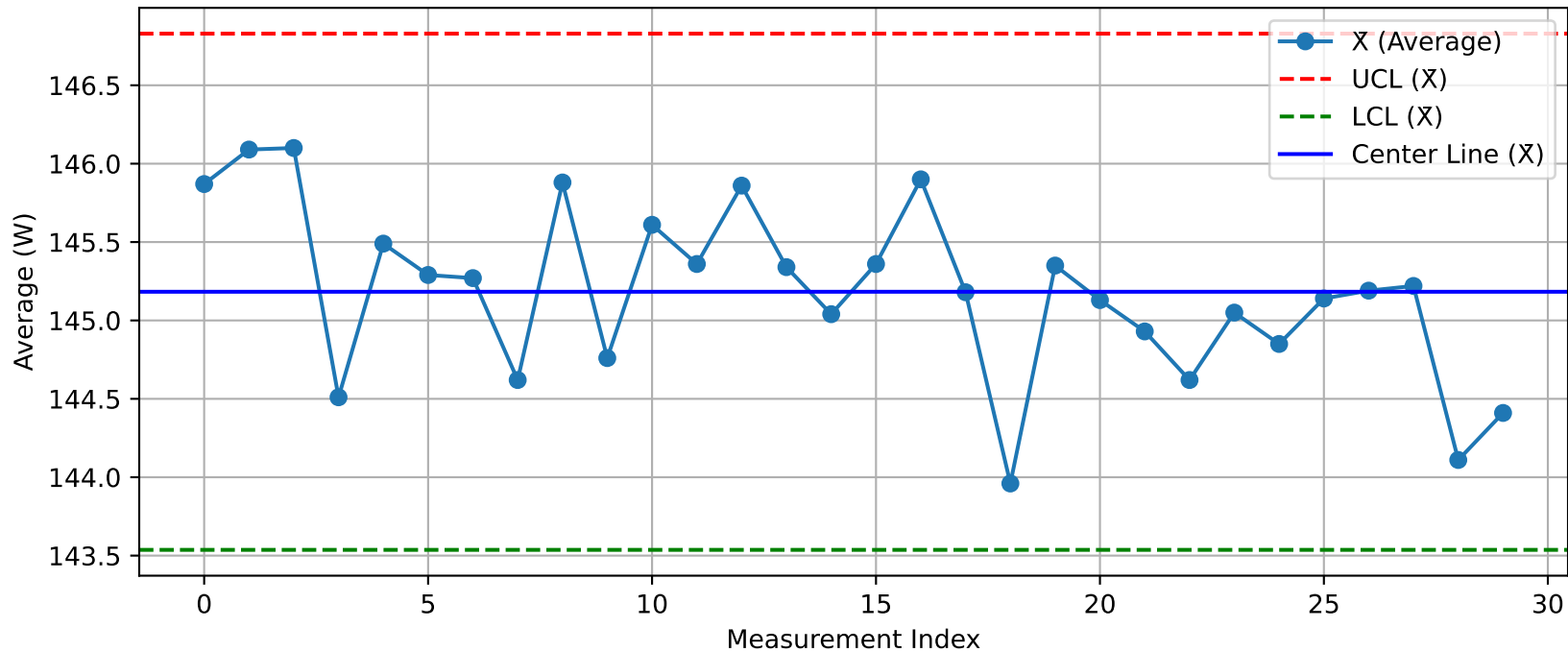
DUT - \bar{X} Chart (T20_Test2_Xint@Test.xlsx)
