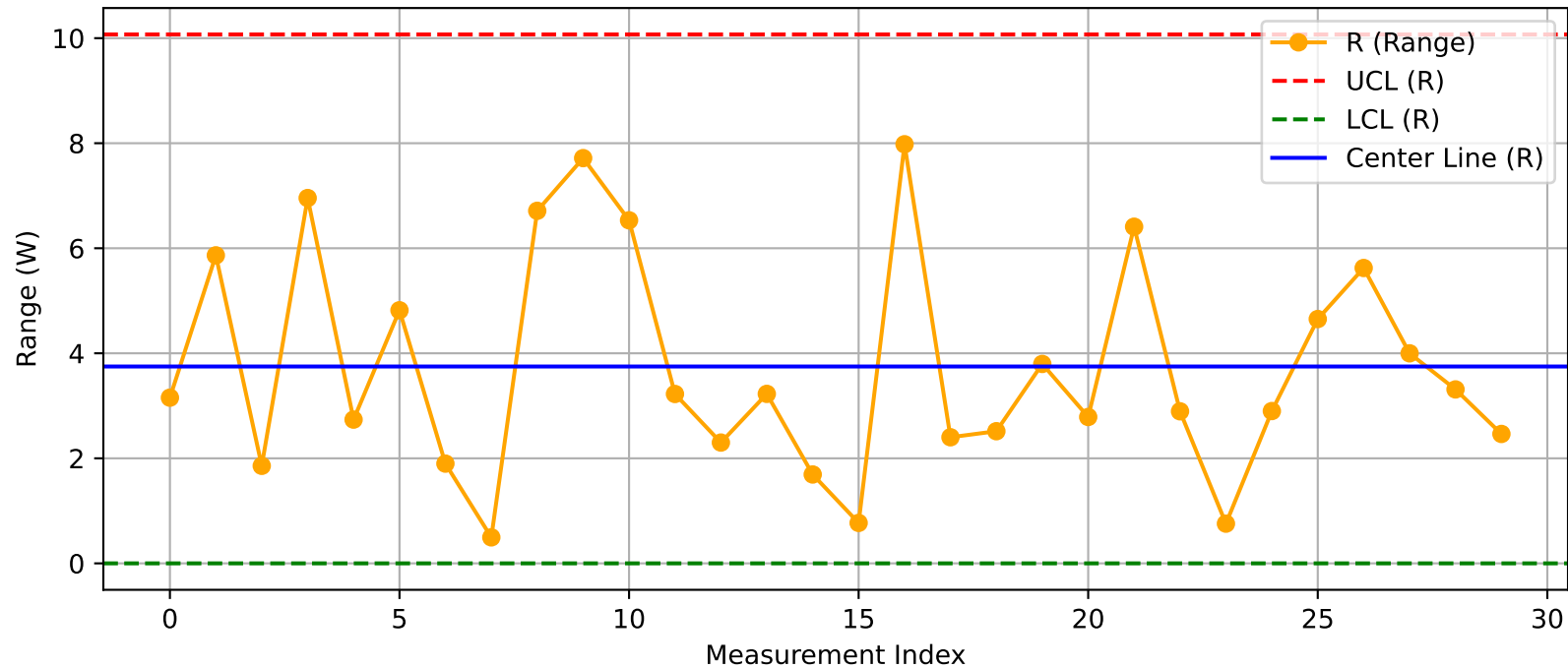
DUT - R Chart (T25_Test2@Test.xlsx)
