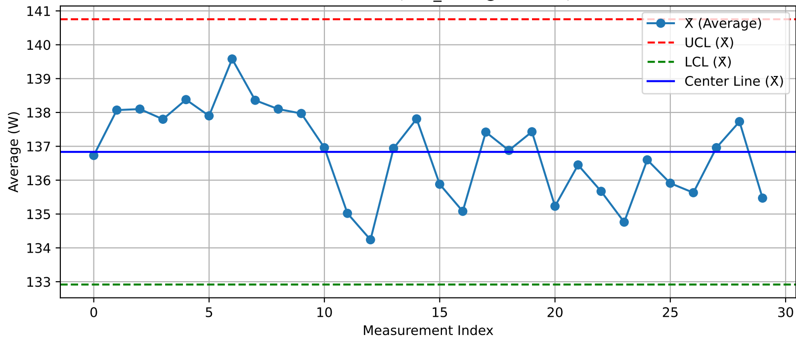
DUT - \bar{X} Chart (T25_Test2@Test.xlsx)
