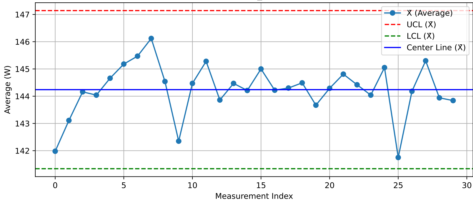
DUT - \bar{X} Chart (T26_Test1@Test.xlsx)
