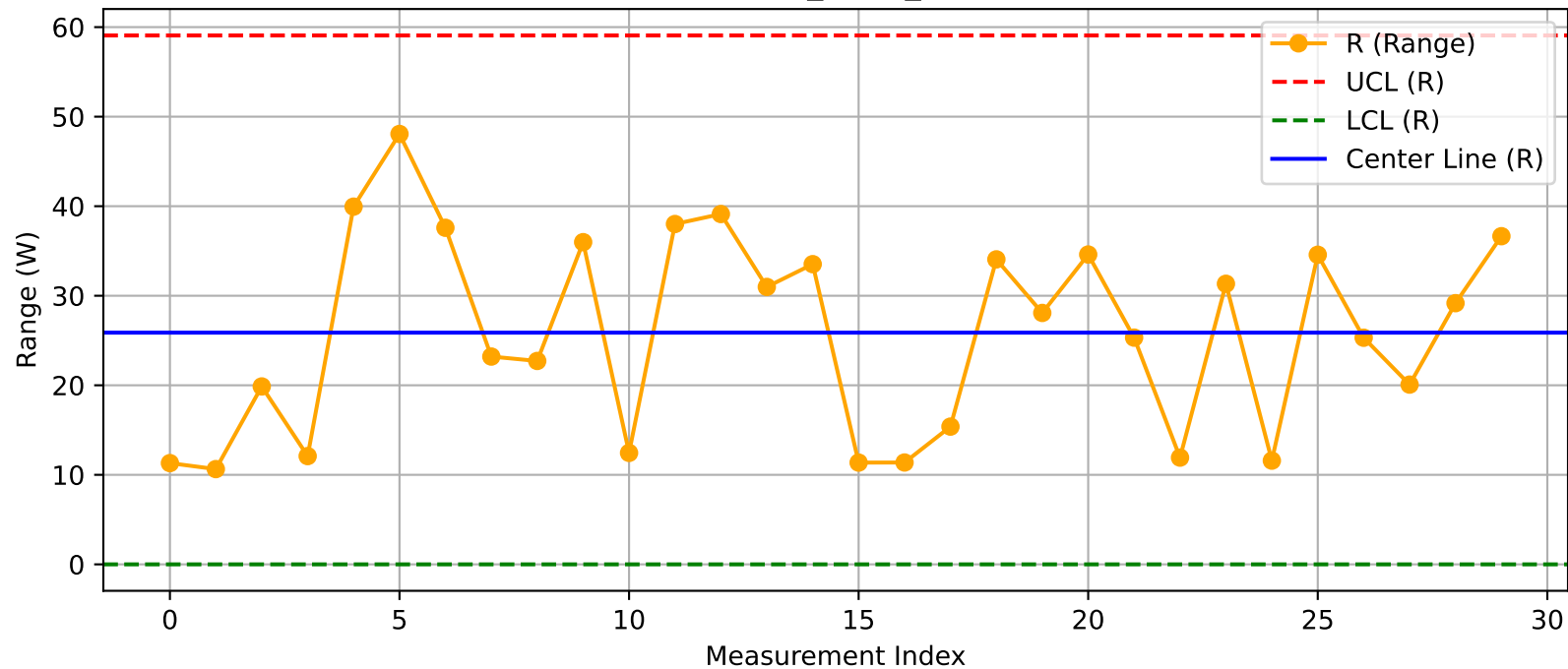
DUT - R Chart (T26_Test2_Xint@Test.xlsx)
