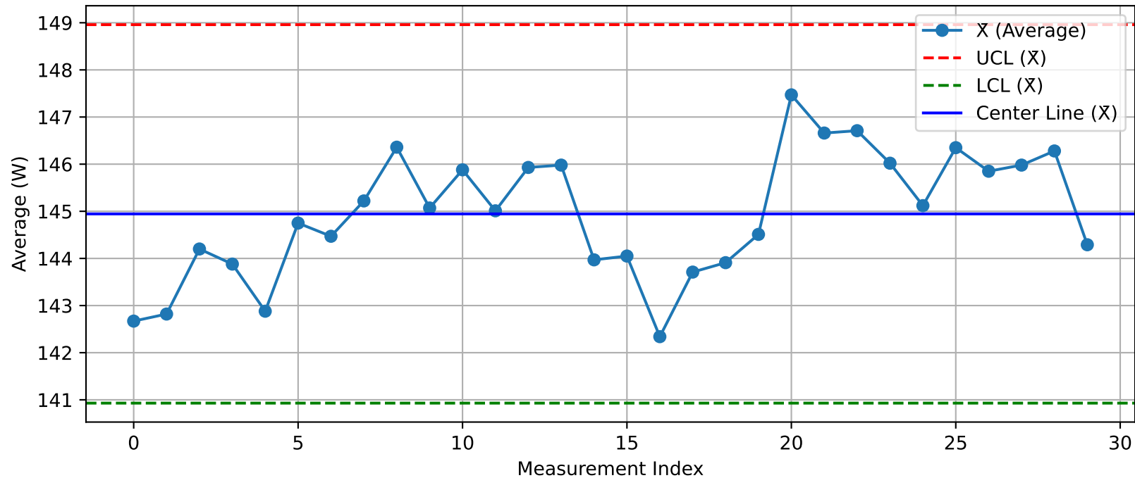
DUT - \bar{X} Chart (T28_Test1_Xint@Test.xlsx)
