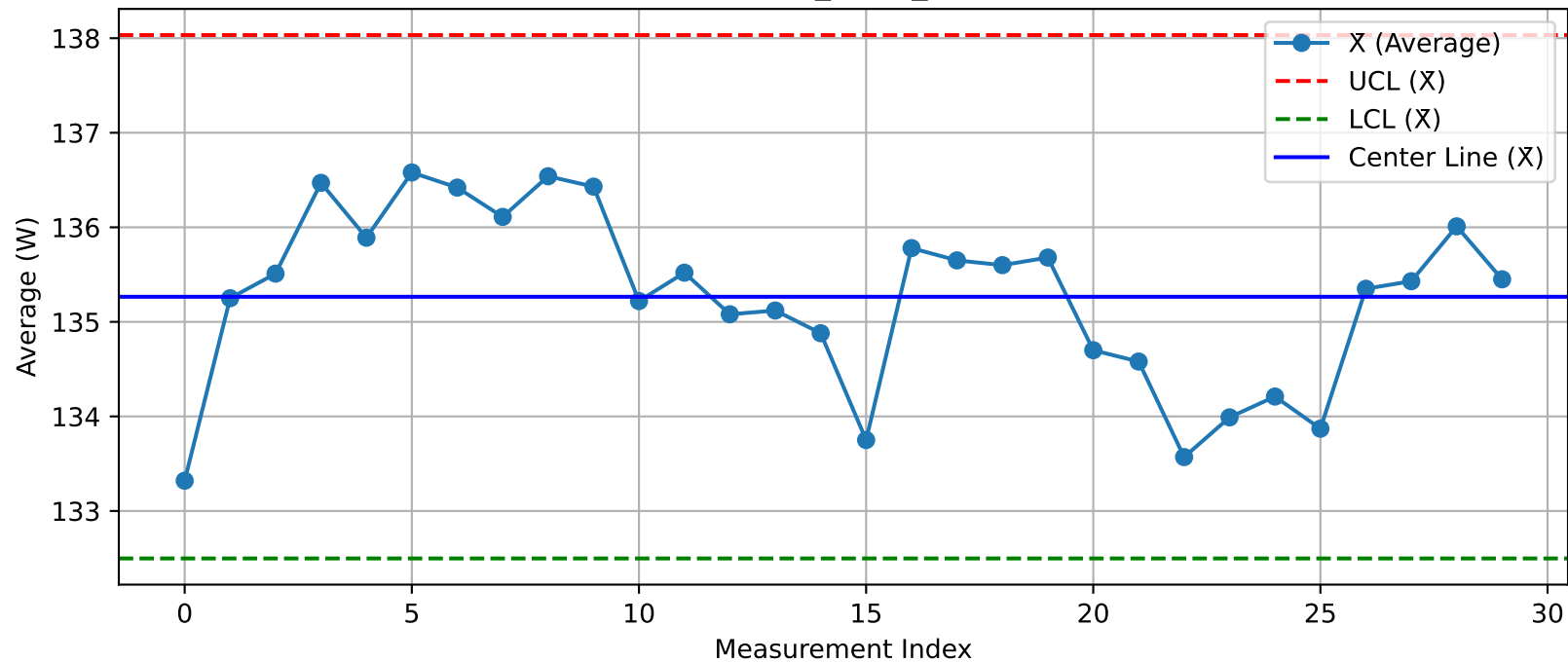
DUT - X Chart (T31_Test1_Xint@Test.xlsx)
