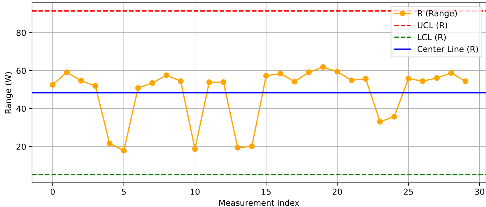
DUT - R Chart (T31_Test2@Test.xlsx)
