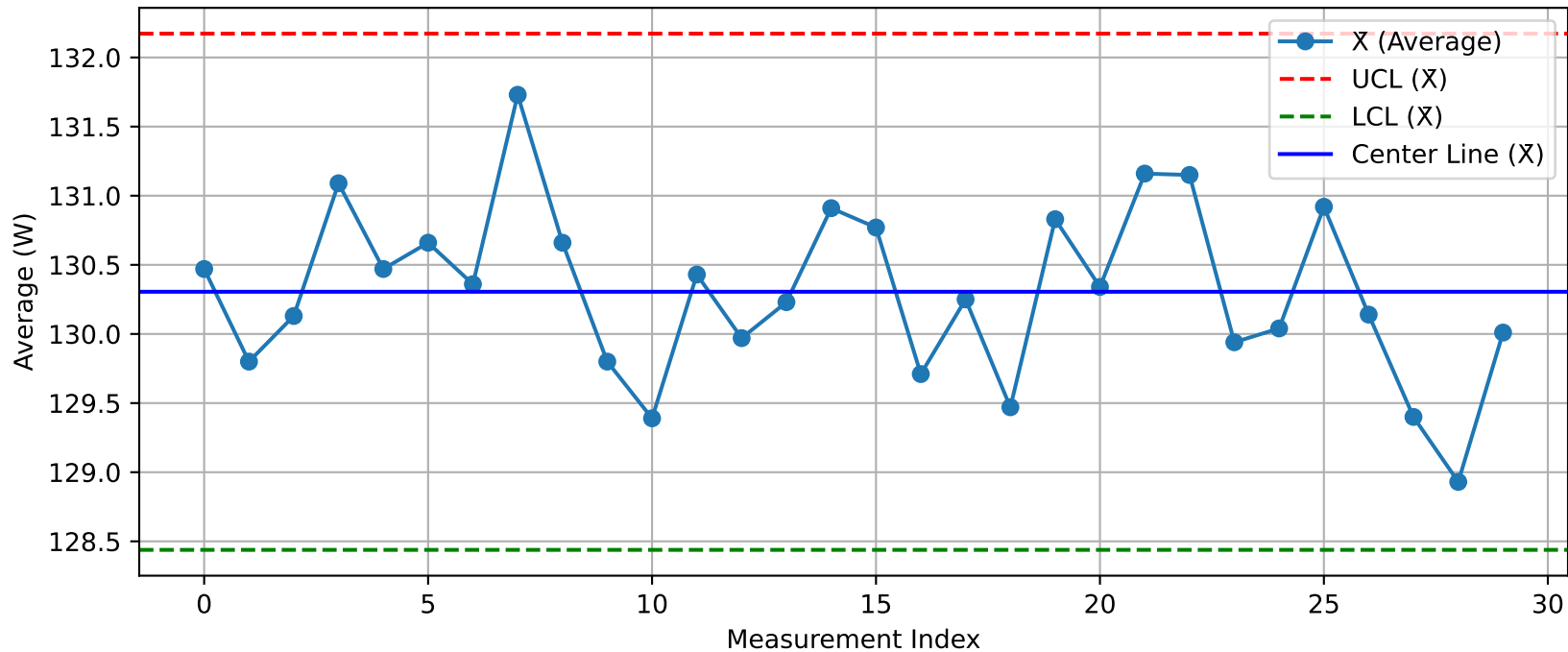
DUT - \bar{X} Chart (T33_Test2_Xint@Test.xlsx)
