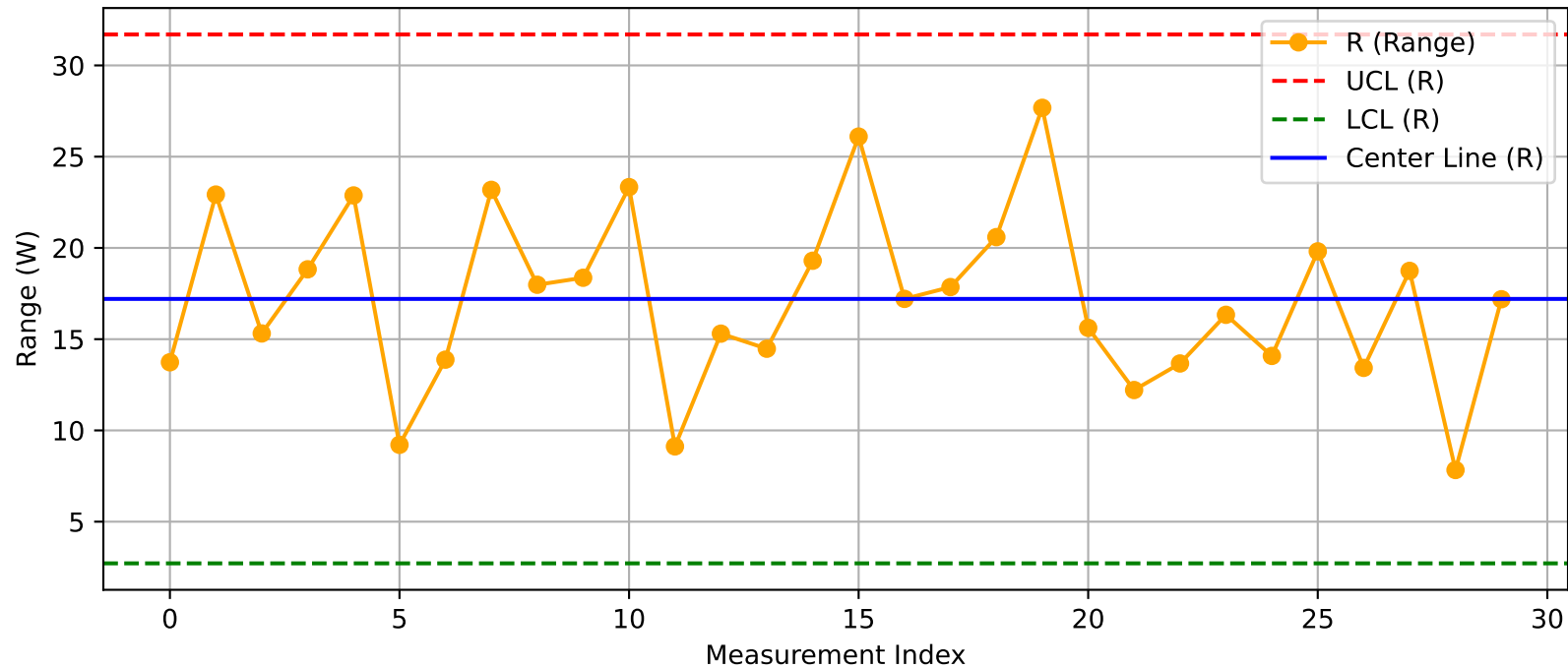
DUT - R Chart (T40_Test2_Xint@Test.xlsx)
