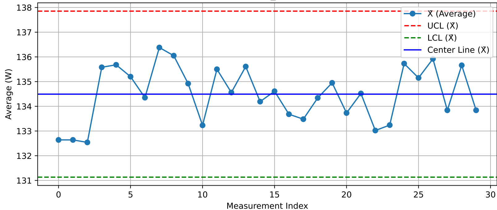
DUT - \bar{X} Chart (T44_Test1@Test.xlsx)
