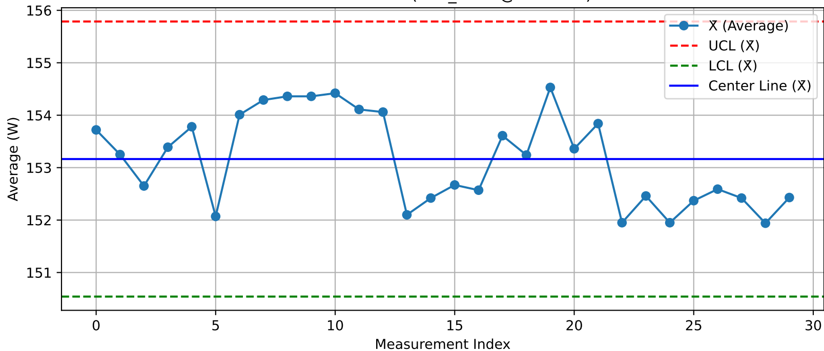
DUT - \bar{X} Chart (T49_Test1@Test.xlsx)
