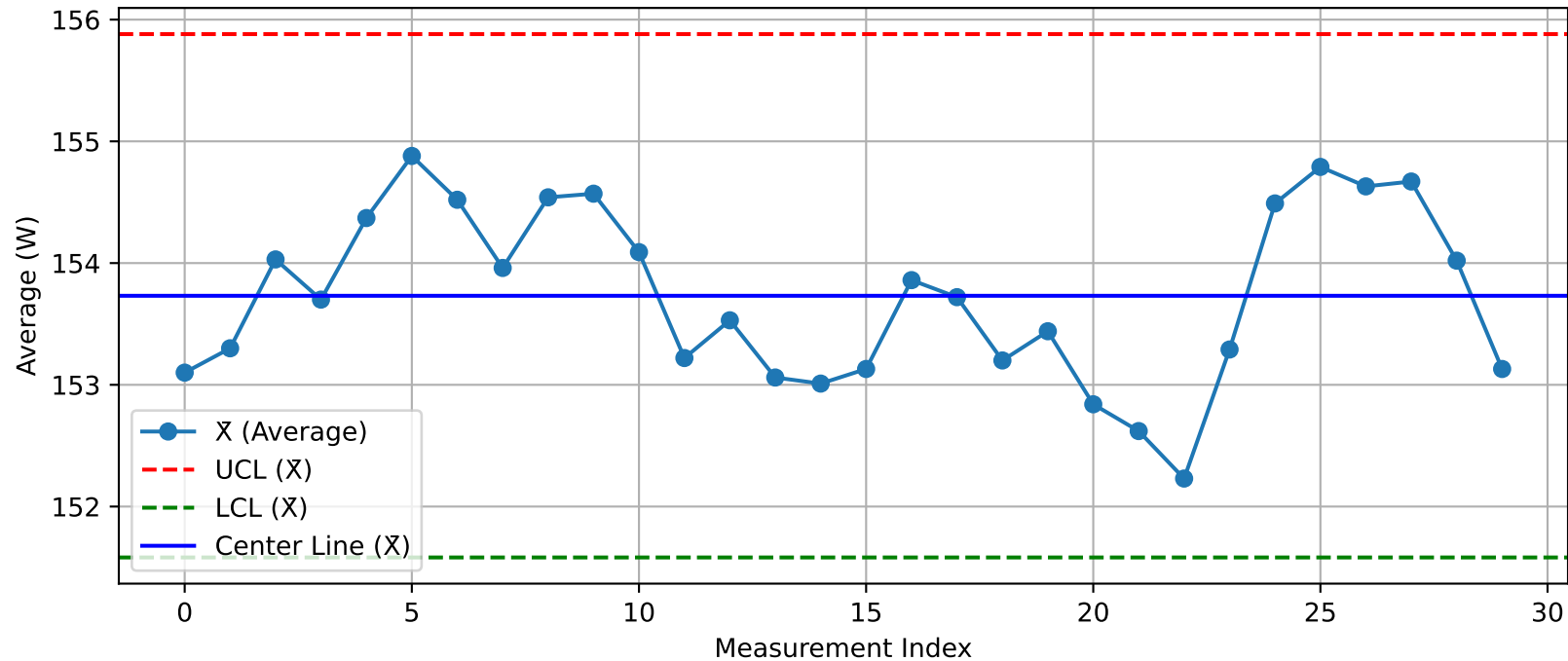
DUT - \bar{X} Chart (T49_Test2@Test.xlsx)
