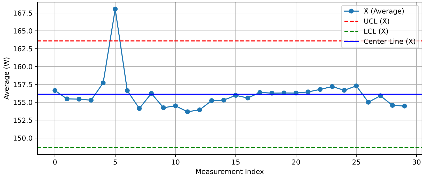
DUT - X Chart (T49_Test2_Xint@Test.xlsx)
