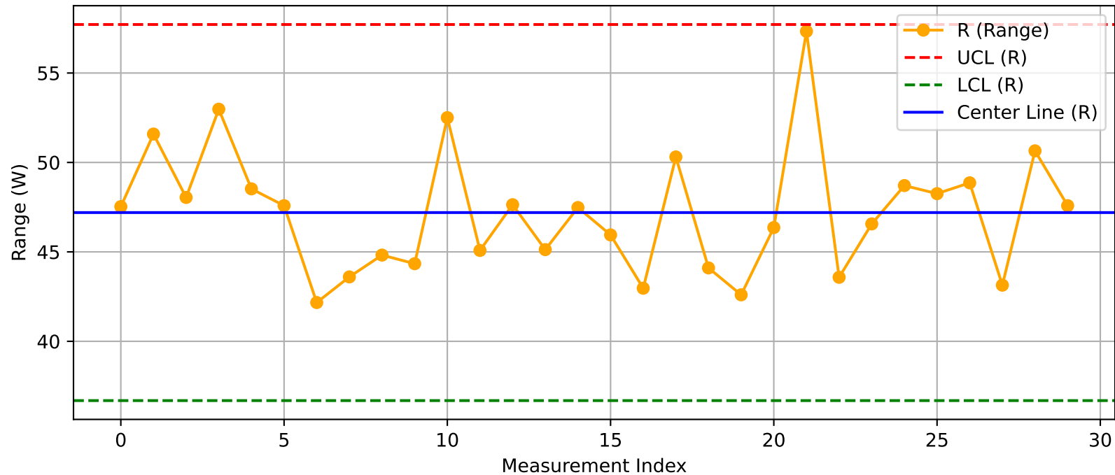
DUT - R Chart (T4_Test1_Xint@Test.xlsx)
