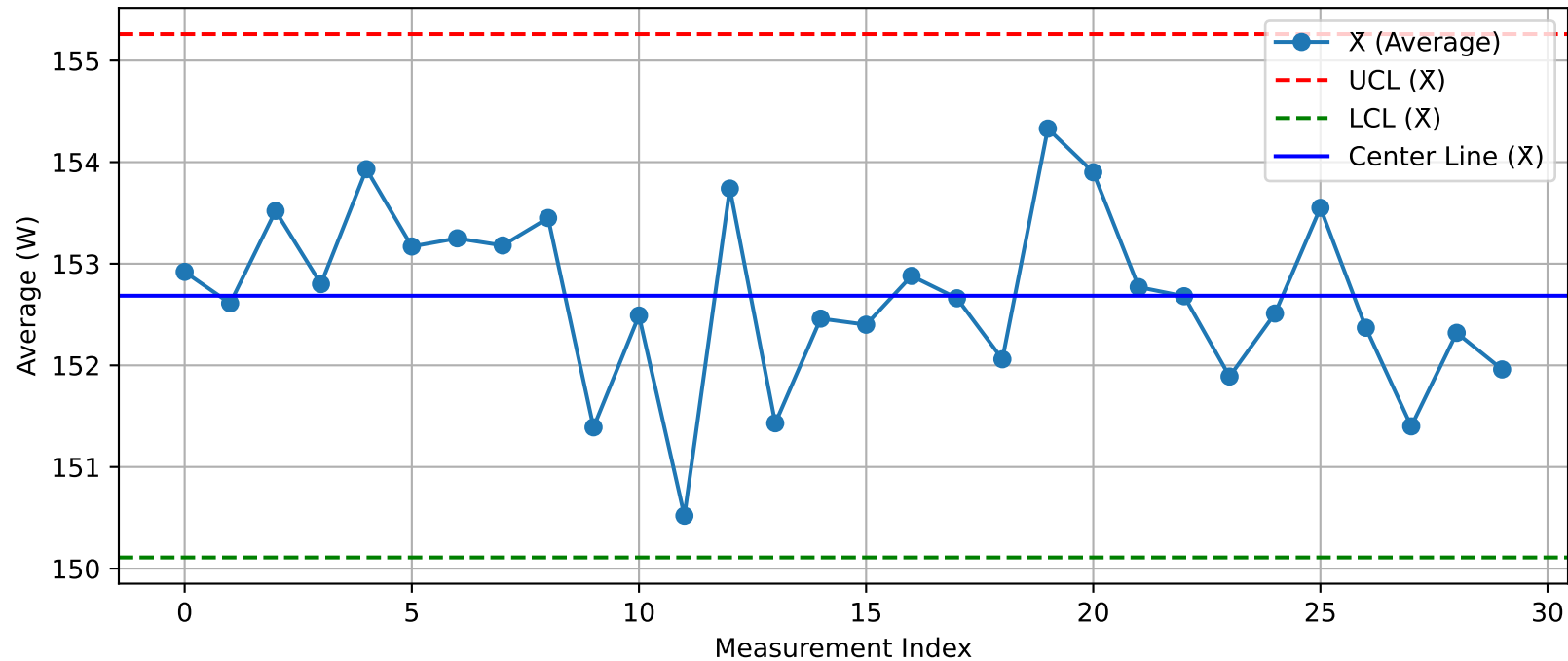
DUT - \bar{X} Chart (T4_Test1_Xint@Test.xlsx)
