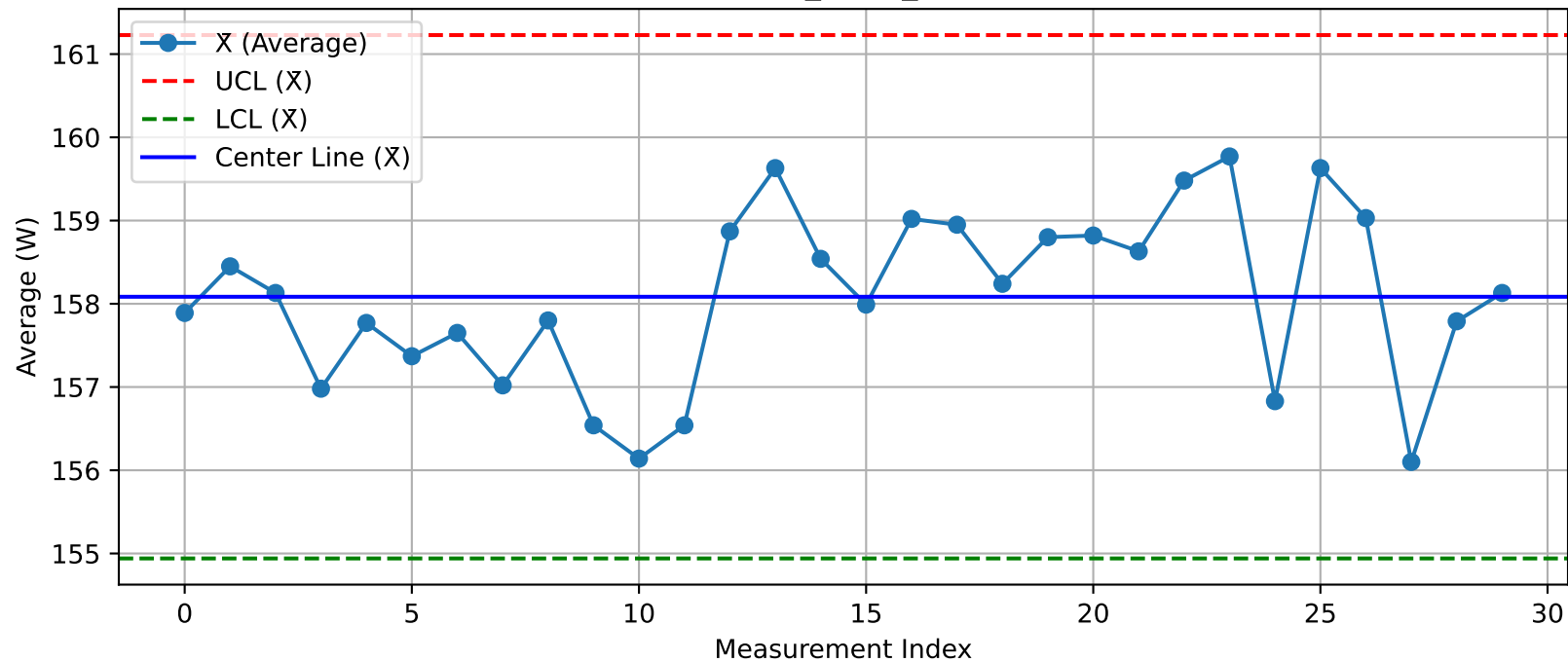
DUT - \bar{X} Chart (T4_Test2_Xint@Test.xlsx)
