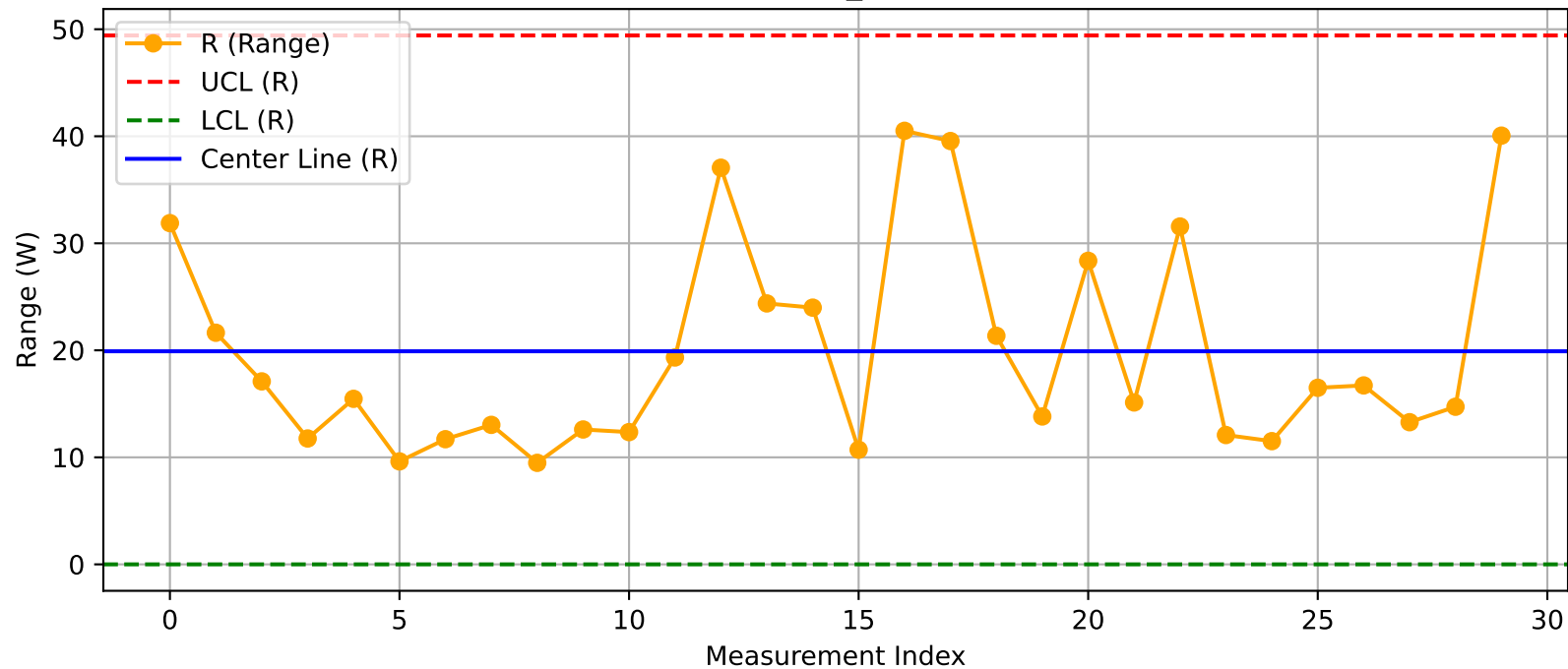
DUT - R Chart (T51_Test2@Test.xlsx)
