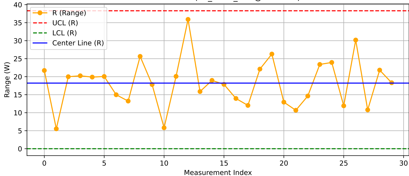
DUT - R Chart (T7_Test1_Xint@Test.xlsx)
