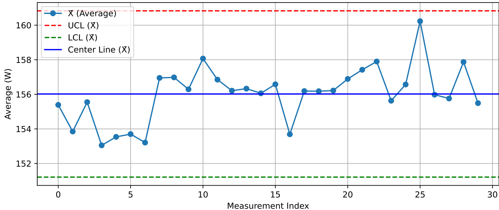
DUT - \bar{X} Chart (T7_Test2@Test.xlsx)
