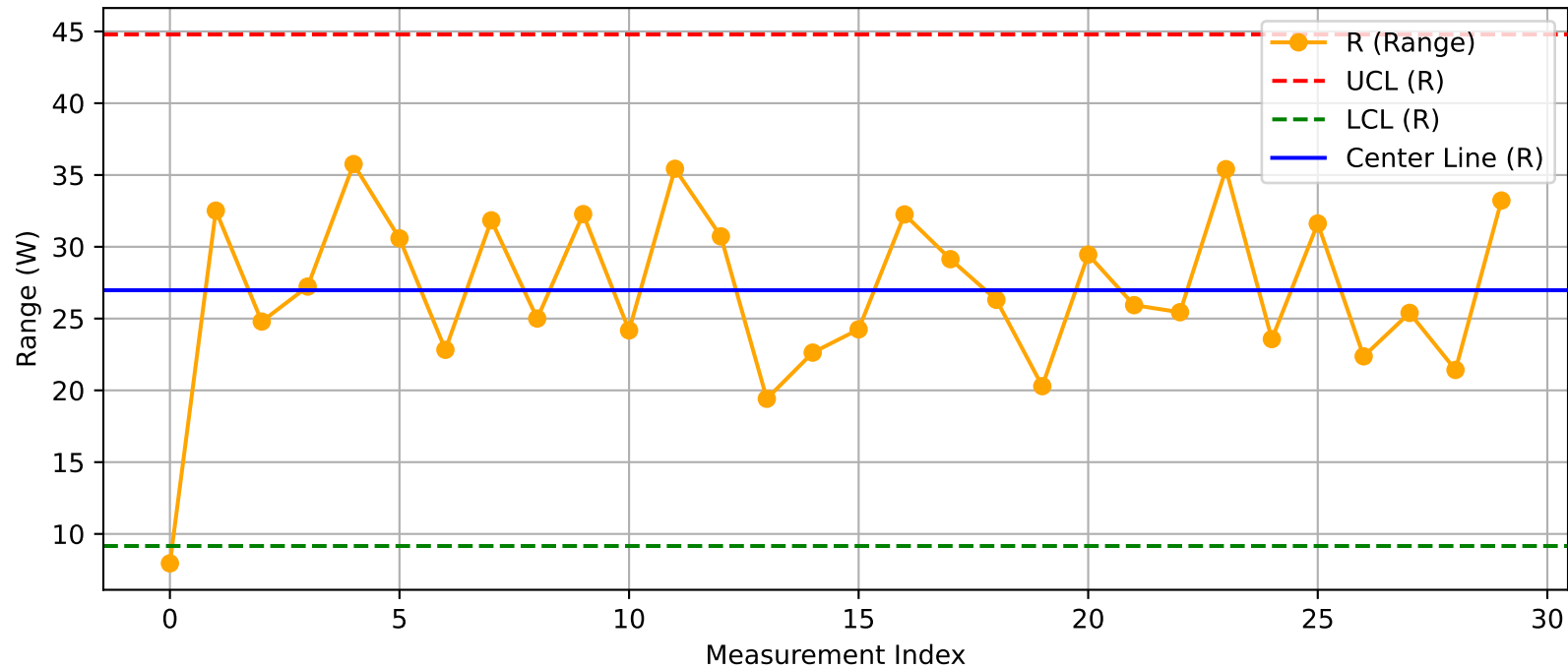
DUT - R Chart (T7_Test2_Xint@Test.xlsx)
