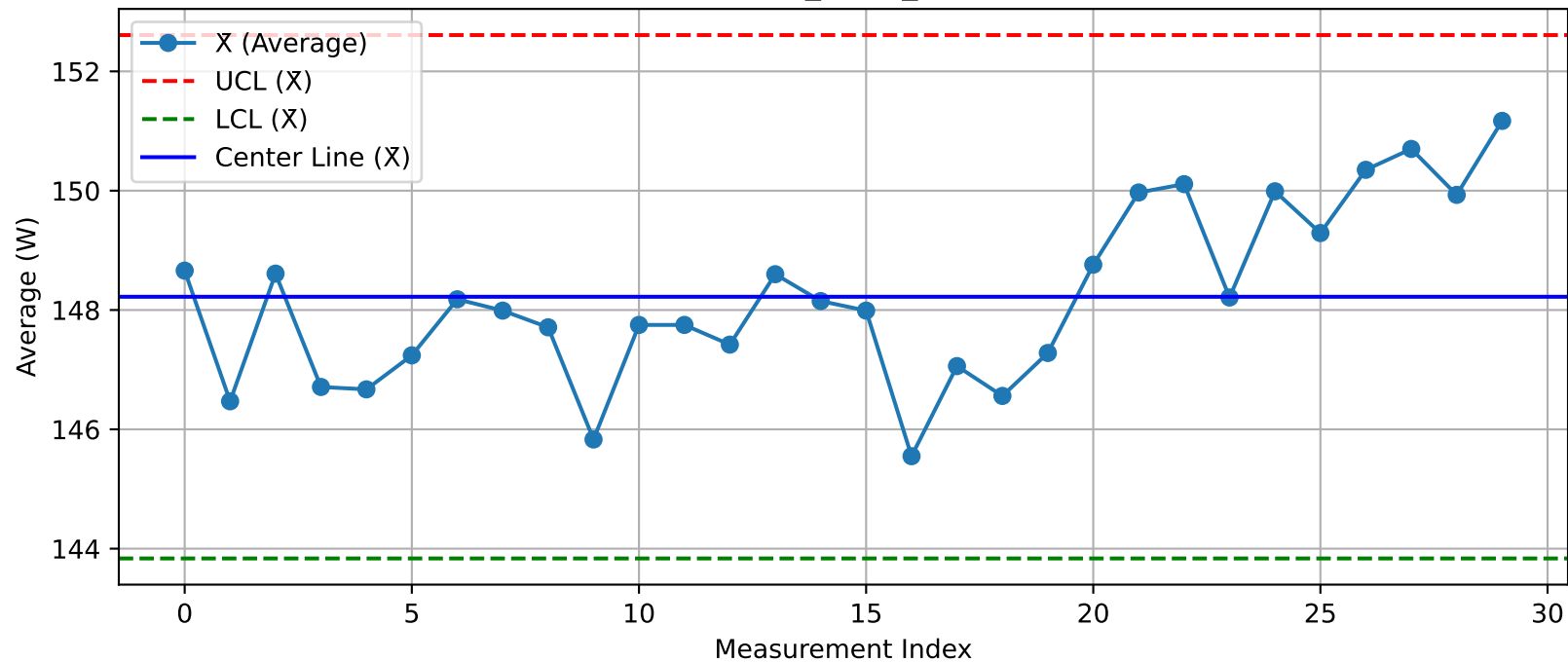
DUT - \bar{X} Chart (T7_Test2_Xint@Test.xlsx)
