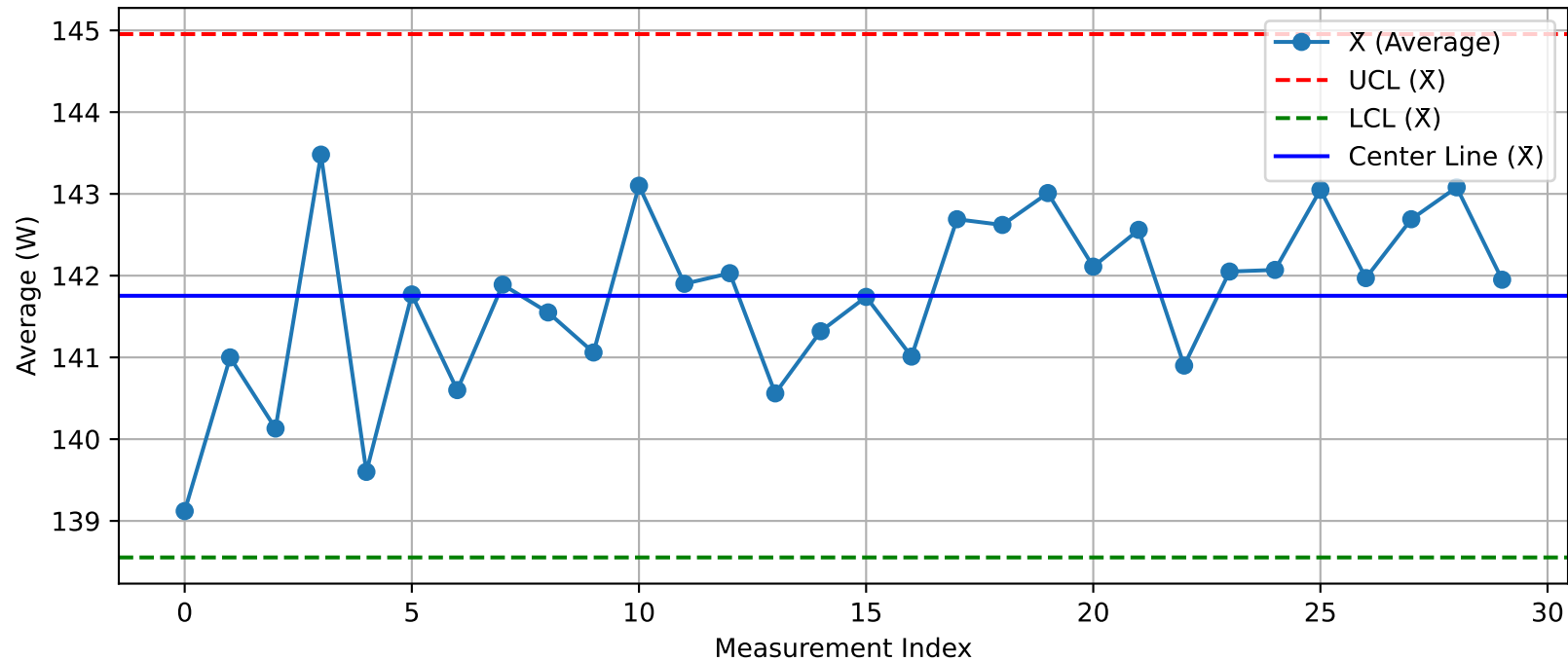
DUT - \bar{X} Chart (T9_Test1@Test.xlsx)
