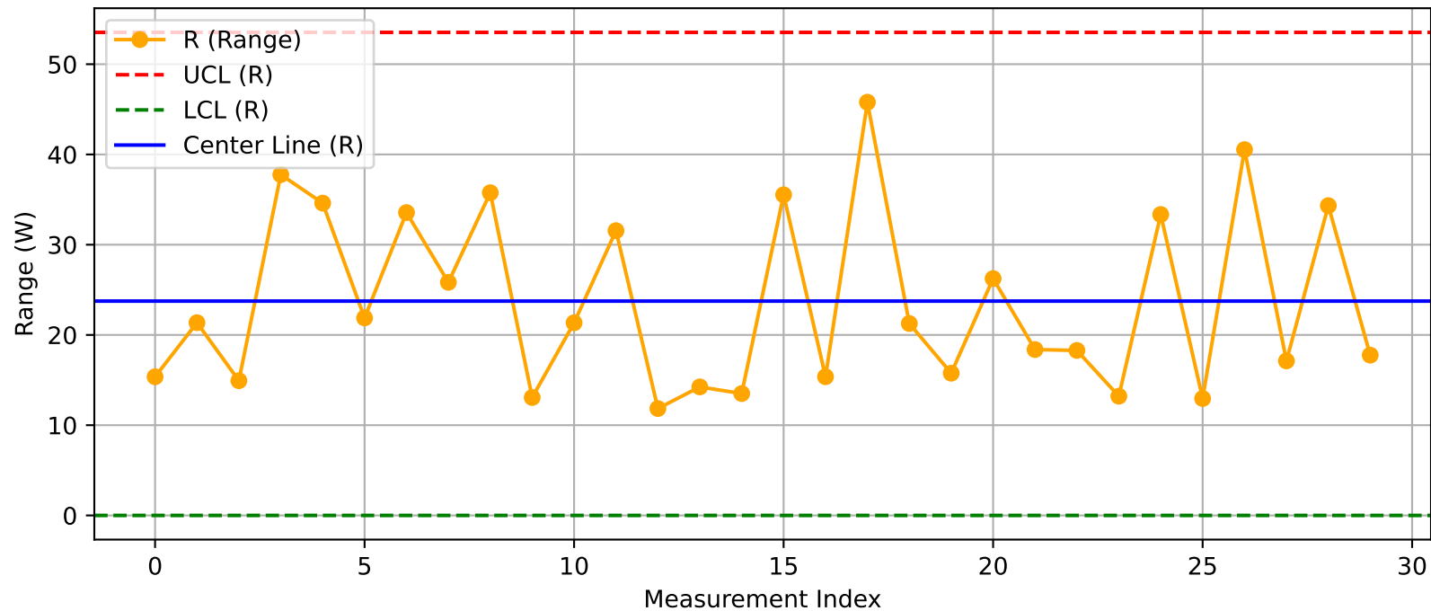
DUT - R Chart (T11@Test1.xlsx)
