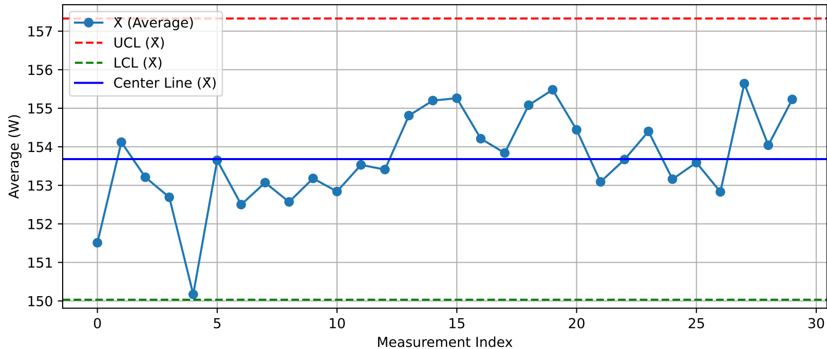
DUT - \bar{X} Chart (T11@Test1.xlsx)
