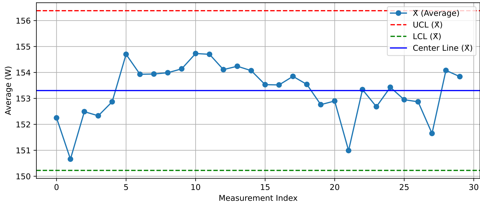
DUT - \bar{X} Chart (T11@Test2.xlsx)
