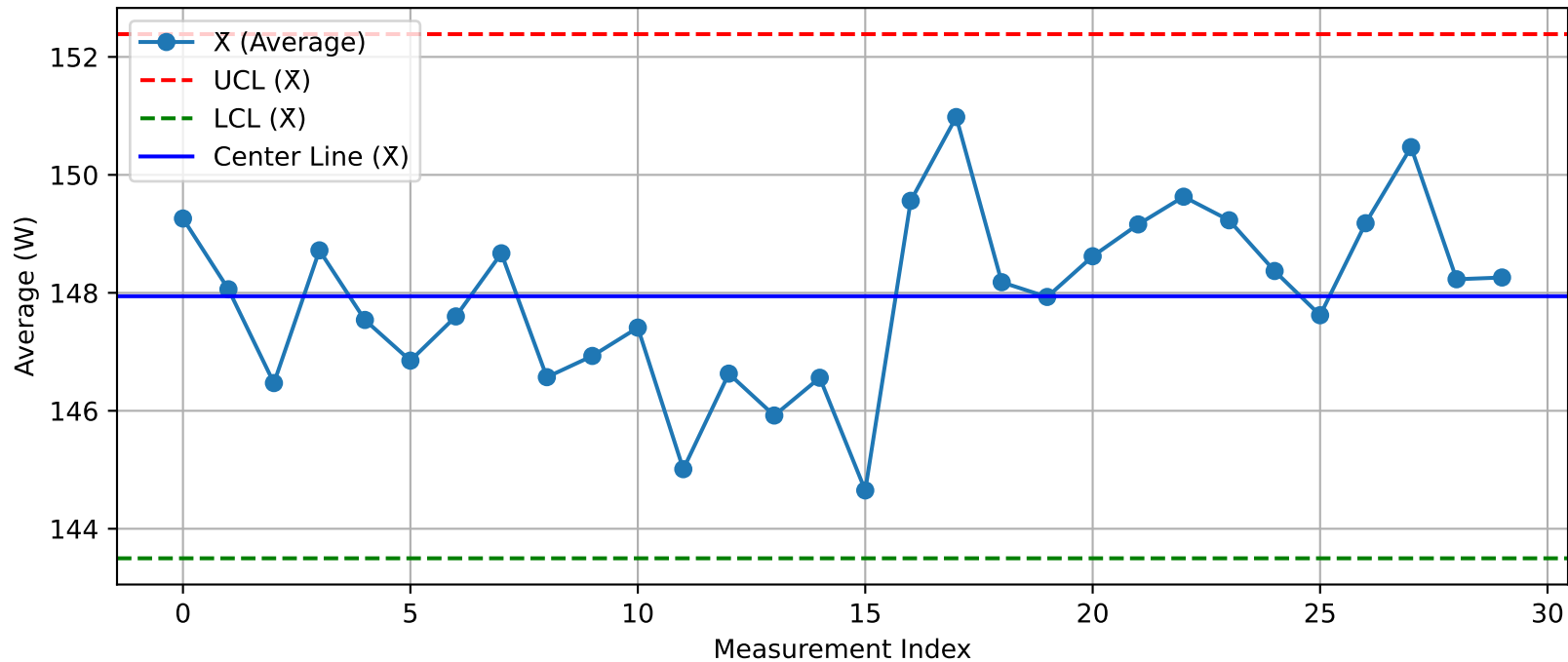
DUT - \bar{X} Chart (T12@Test2.xlsx)
