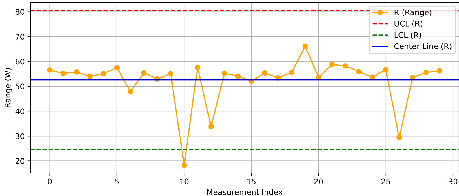
DUT - R Chart (T13@Test1_Nuitka.xlsx)
