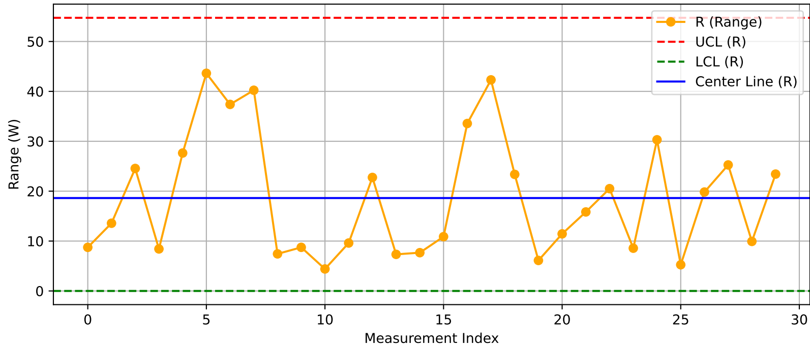
DUT - R Chart (T16@Test1_Nuitka.xlsx)
