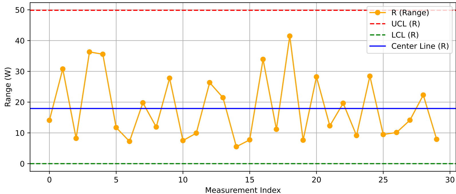
DUT - R Chart (T16@Test2.xlsx)
