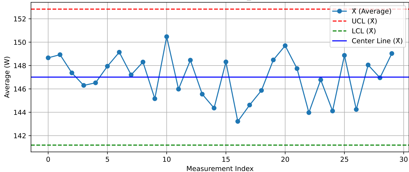
DUT - \bar{X} Chart (T17@Test1_Nuitka.xlsx)
