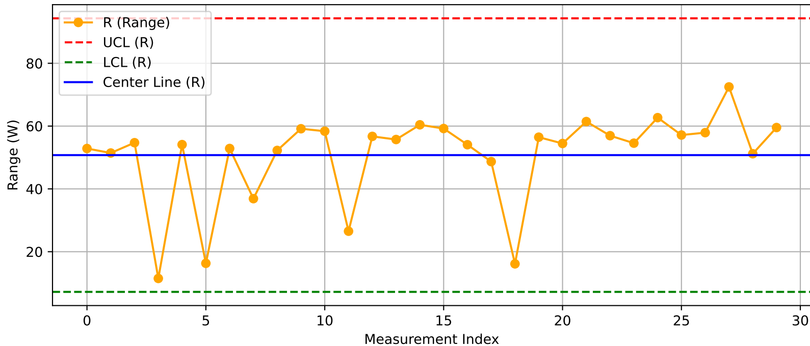
DUT - R Chart (T19@Test1.xlsx)
