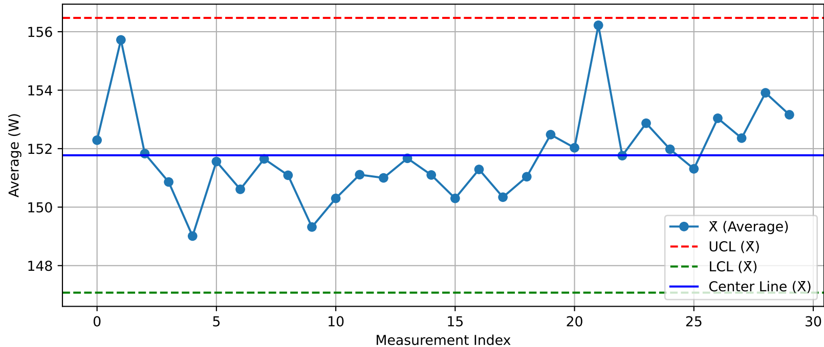
DUT - \bar{X} Chart (T19@Test1_Nuitka.xlsx)
