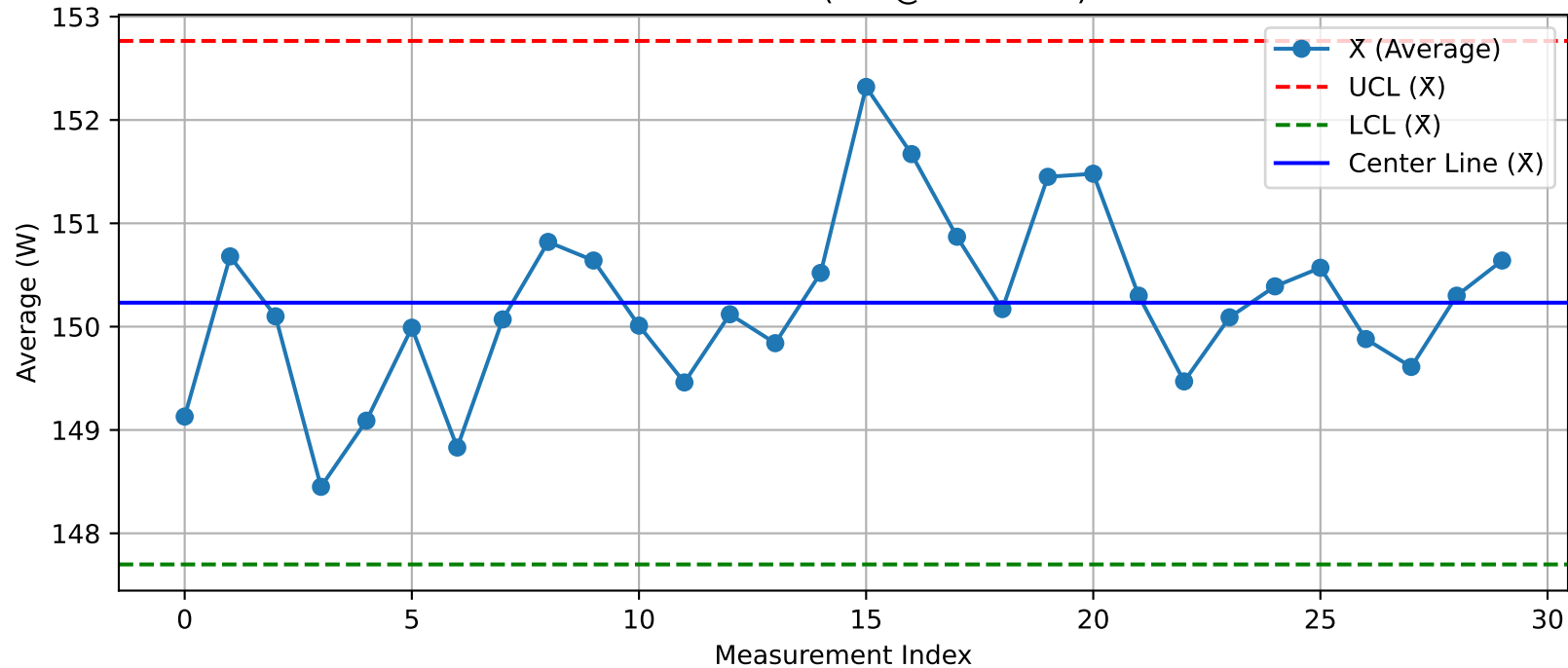
DUT - \bar{X} Chart (T25@Test1.xlsx)
