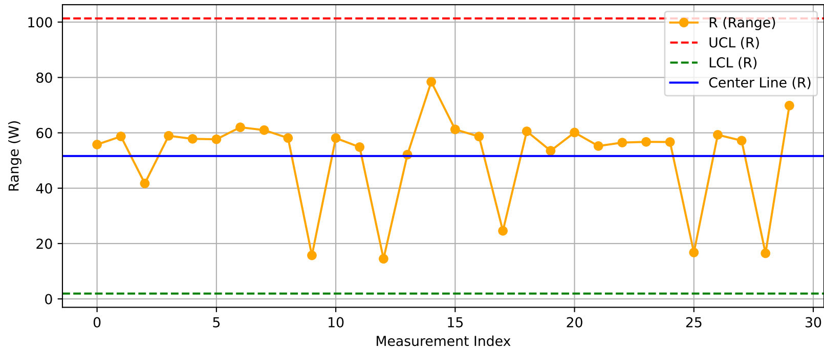
DUT - R Chart (T26@Test1.xlsx)
