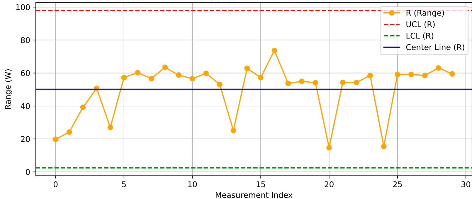
DUT - R Chart (T26@Test1_Nuitka.xlsx)
