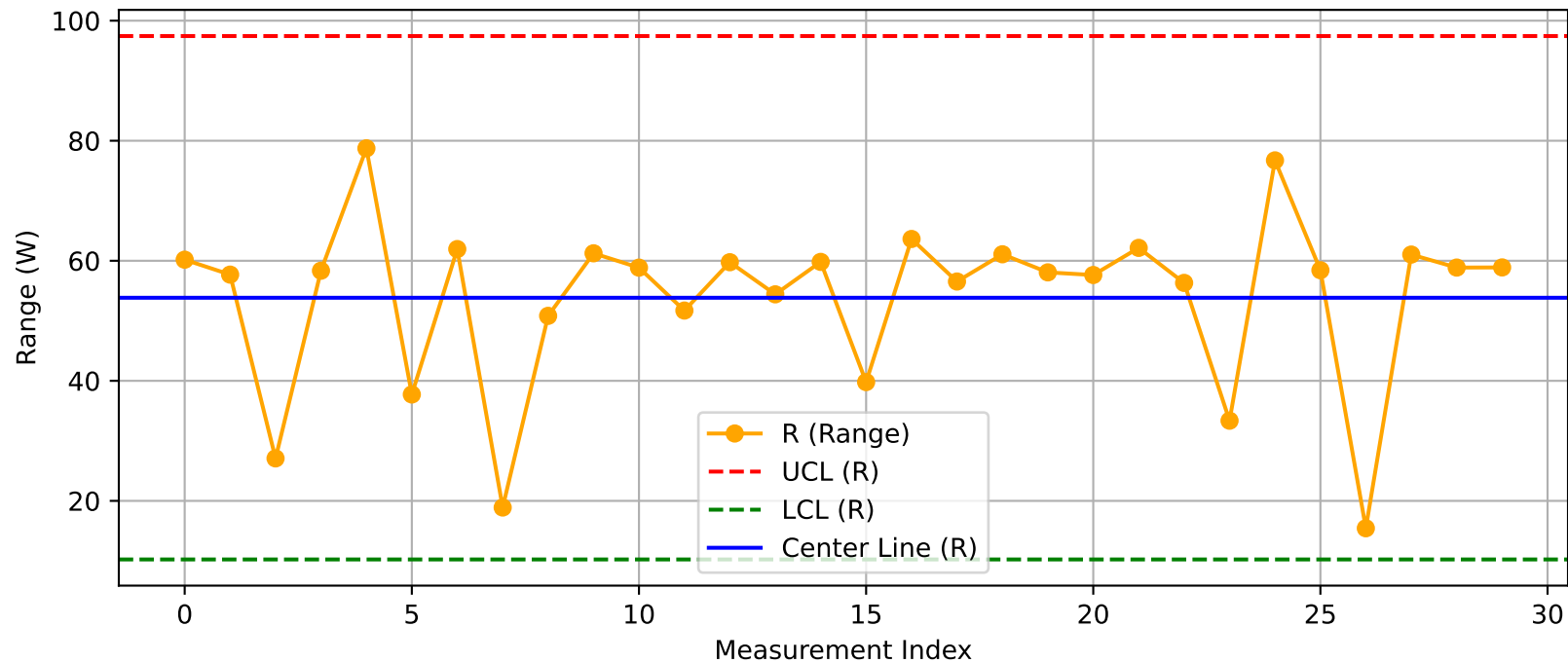
DUT - R Chart (T26@Test2.xlsx)
