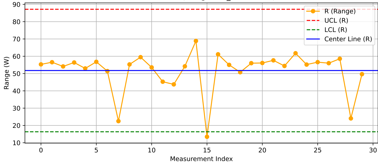
DUT - R Chart (T26@Test2_Nuitka.xlsx)
