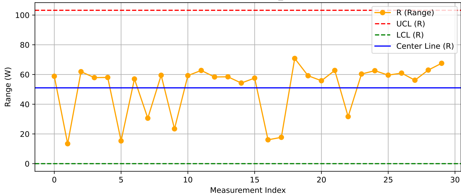
DUT - R Chart (T28@Test2_Nuitka.xlsx)
