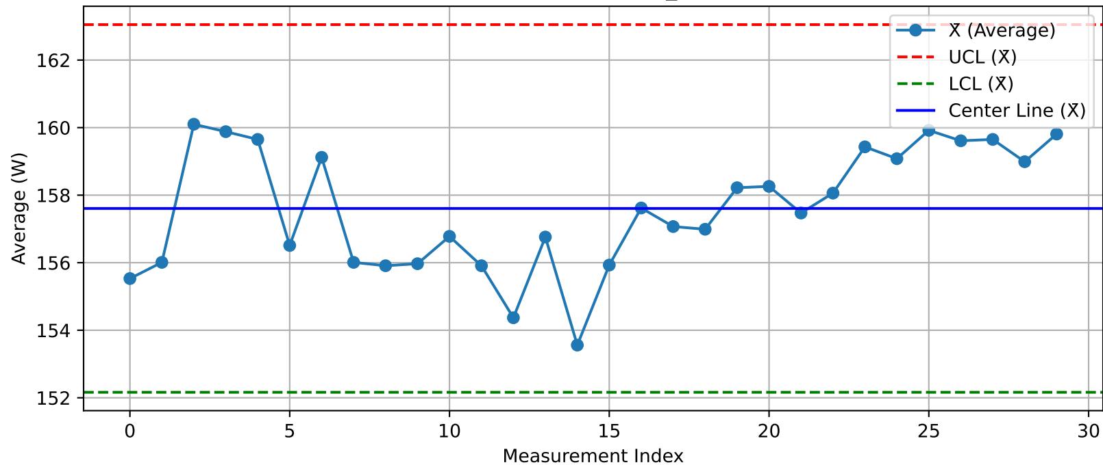
DUT - \bar{X} Chart (T31@Test1_Nuitka.xlsx)
