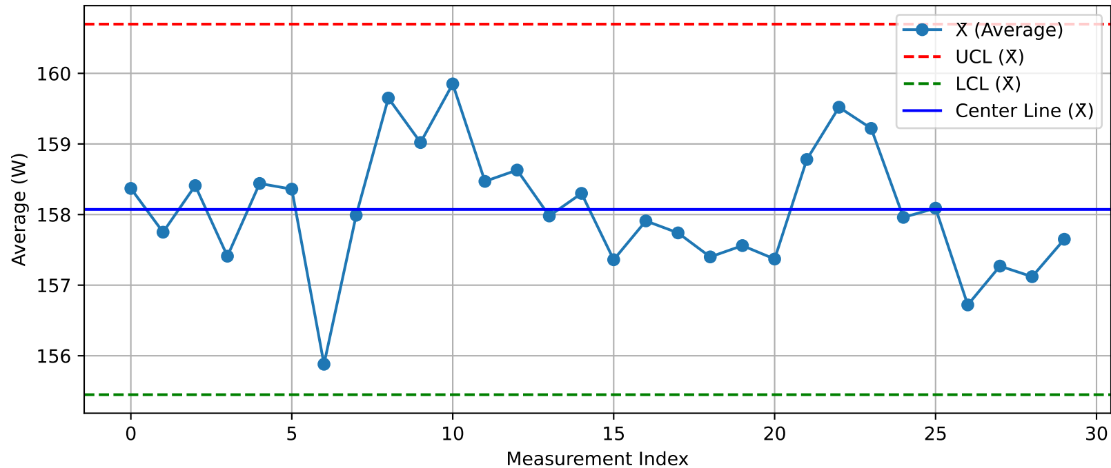
DUT - \bar{X} Chart (T31@Test2_Nuitka.xlsx)
