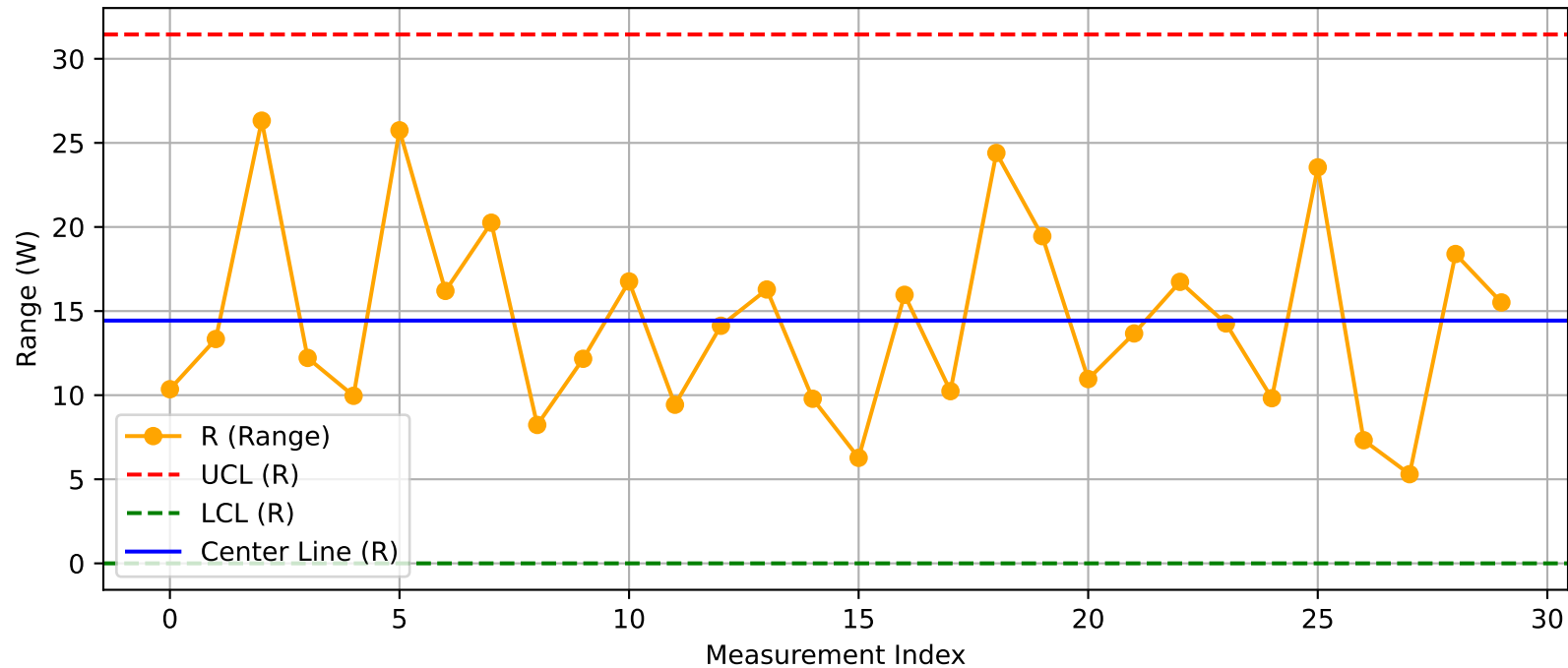
DUT - R Chart (T33@Test1_Nuitka.xlsx)
