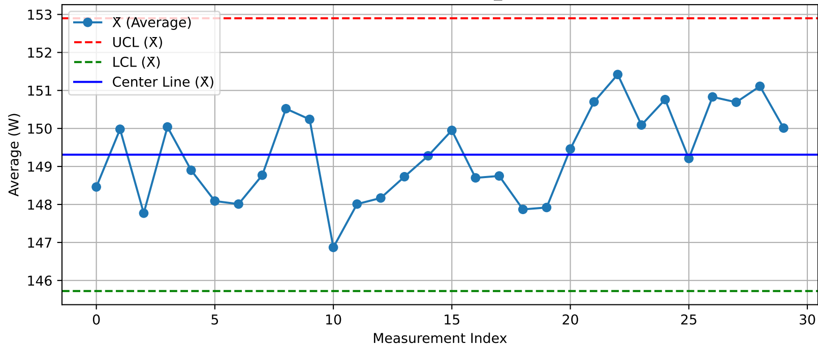
DUT - \bar{X} Chart (T33@Test1_Nuitka.xlsx)
