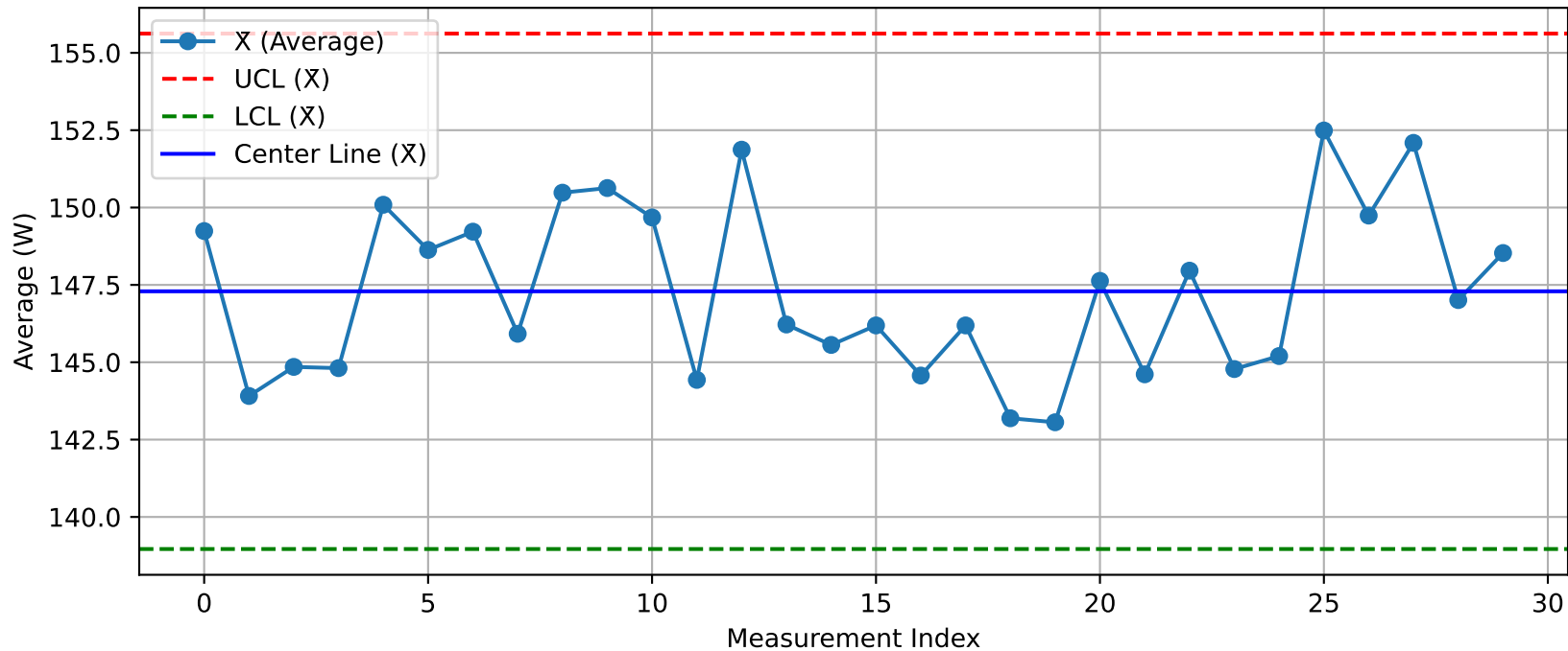
DUT - \bar{X} Chart (T44@Test1_Nuitka.xlsx)
