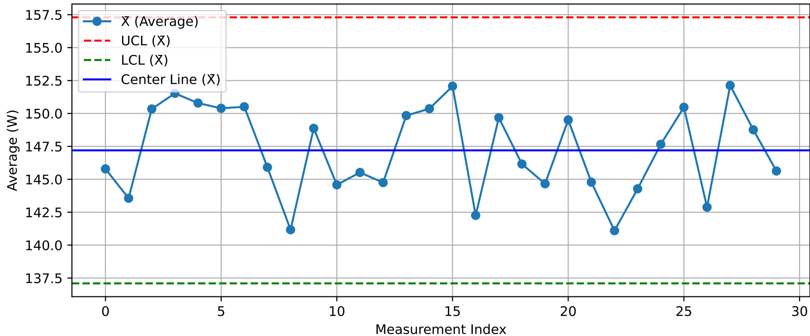
DUT - \bar{X} Chart (T44@Test2_Nuitka.xlsx)
