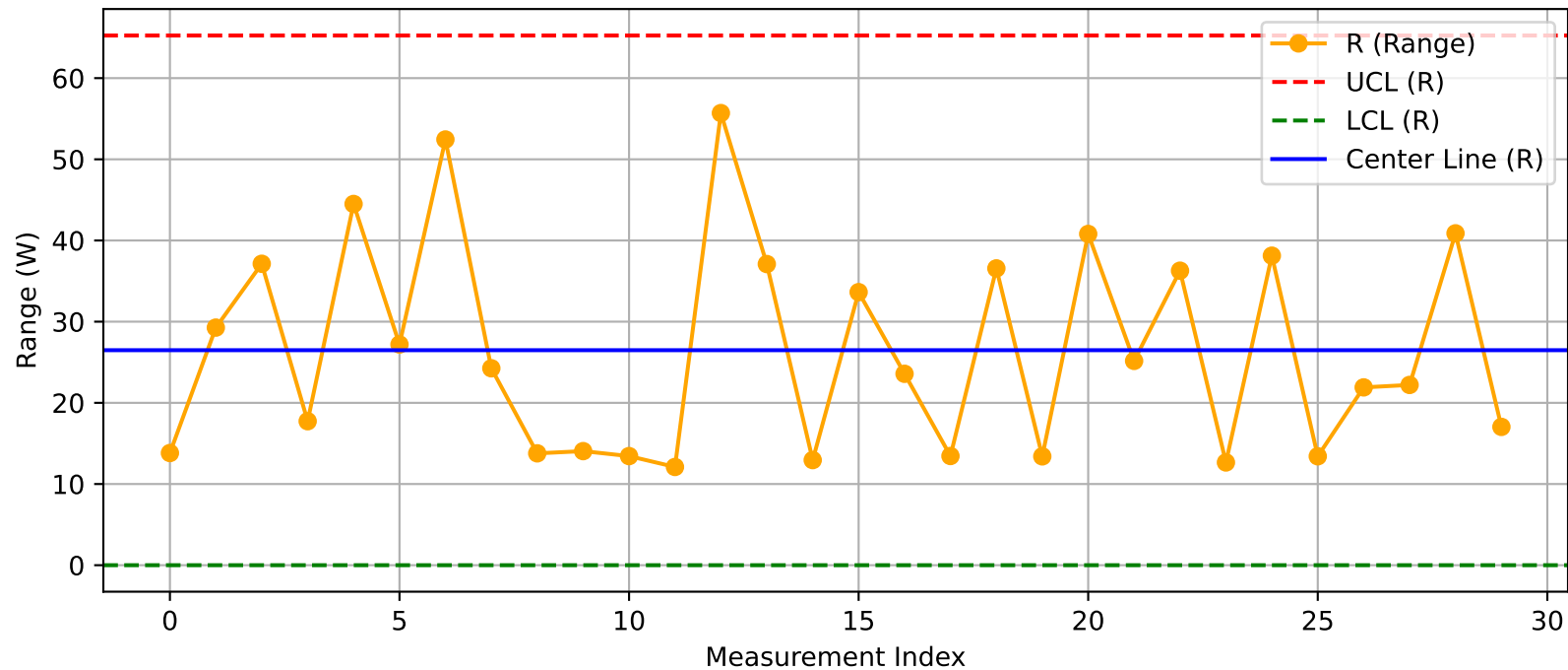
DUT - R Chart (T49@Test1.xlsx)
