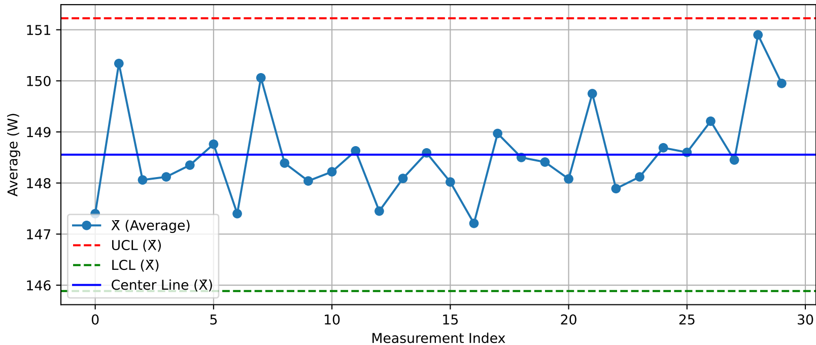
DUT - \bar{X} Chart (T49@Test1.xlsx)
